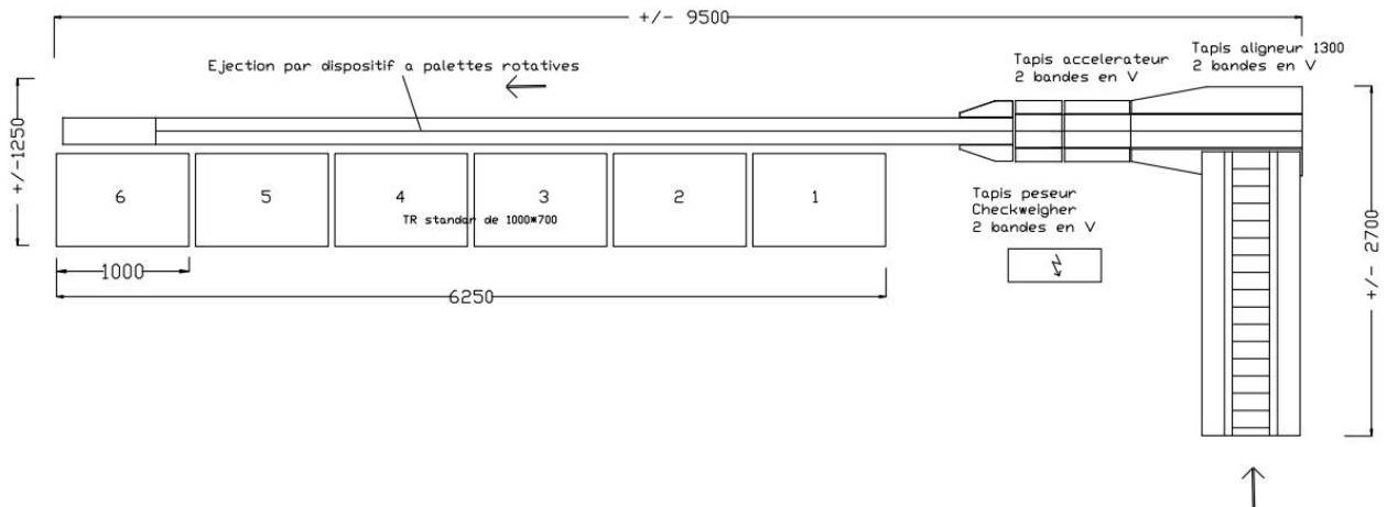
Exemple of a layout of a checkweigher with 7 outputs :
